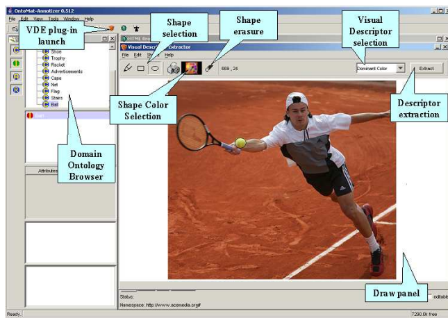
Fig. 4. The VDE plugin into OntoMat-Annotizer tool
