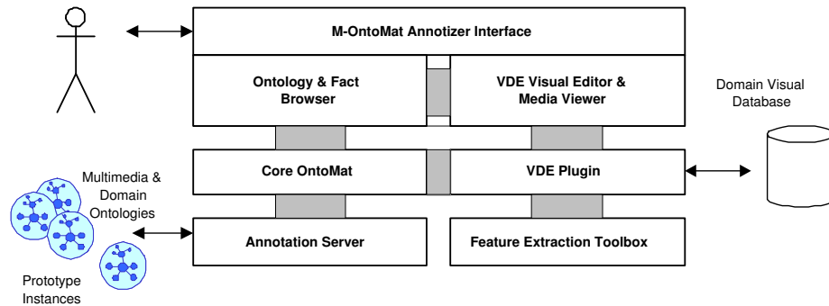
Fig. 3. OntoMat-Annotizer and VDE plug-in design architecture
